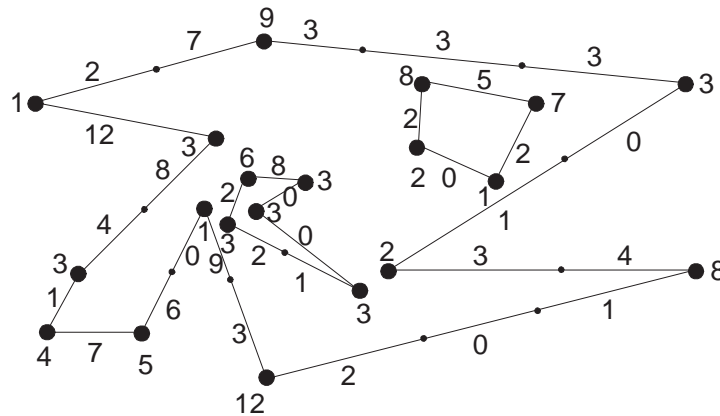
Fig. 2. A weighted polygon with weights on edge segments and costs on vertices
