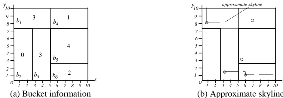
Figure 5.2: Obtaining the approximate skyline for non-uniform data
