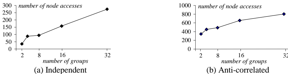
Figure 6.10: BBS node accesses vs. cardinality of categorical axis c_{num} ( N=1M, d=3 )
