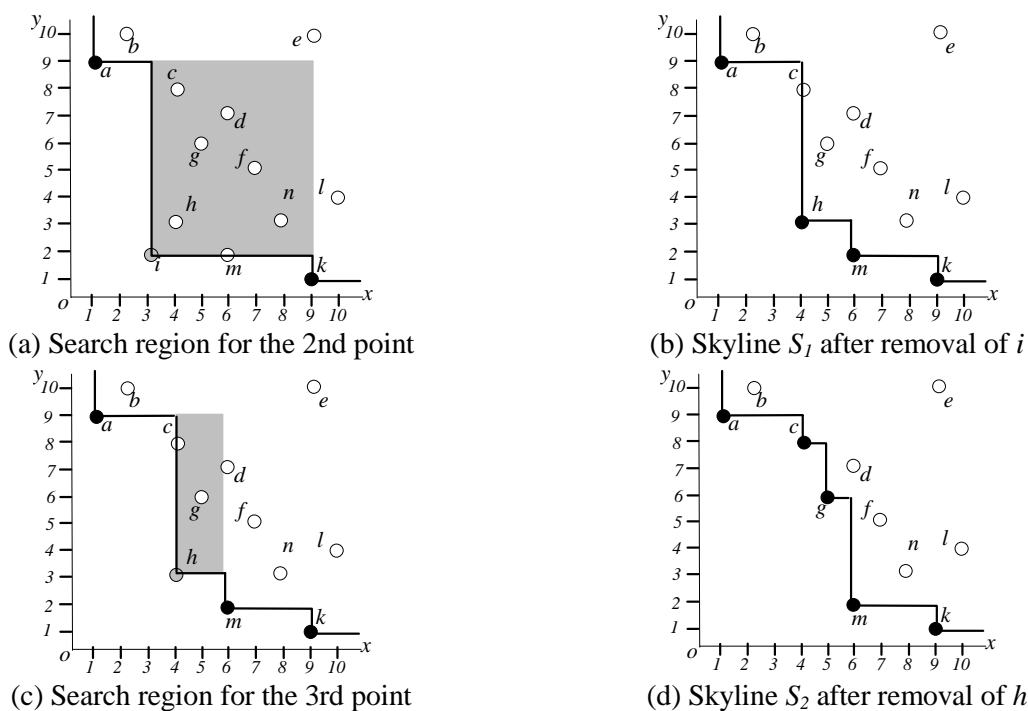
Figure 4.3: Example of 3-dominating query
