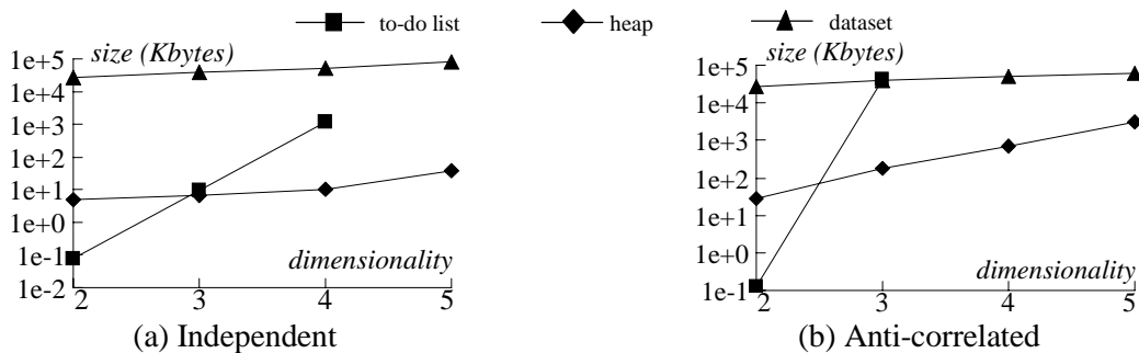
Figure 6.2: Heap and to-do list sizes vs. dimensionality d ( N=1M )
