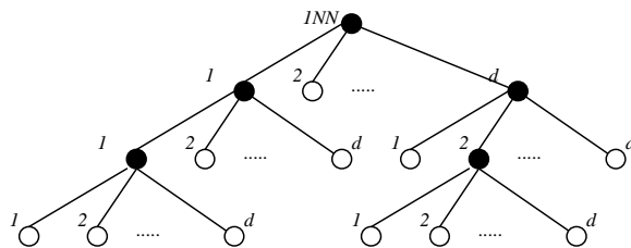
Figure 3.1: Recursion tree
