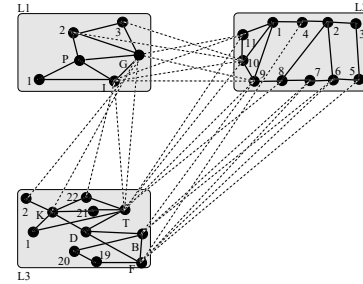
Figure 1: A multilayer network consisting of three layers L1, L2 and L3. Nodes with the same ID in different layers depict clones of the same node.
