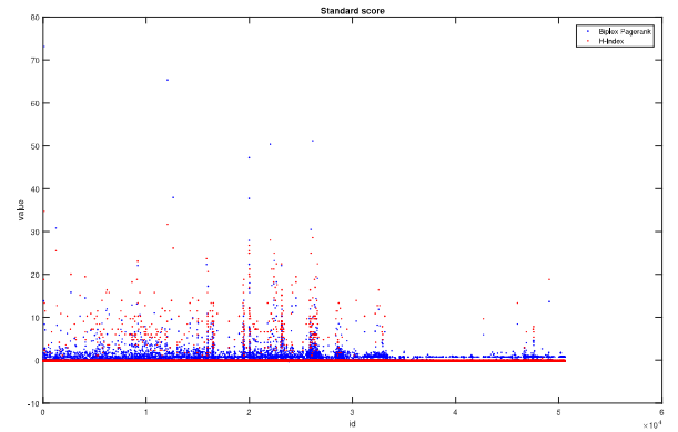
Figure 3: Biplex PageRank versus h -index value distribution and correlation per author ID.
