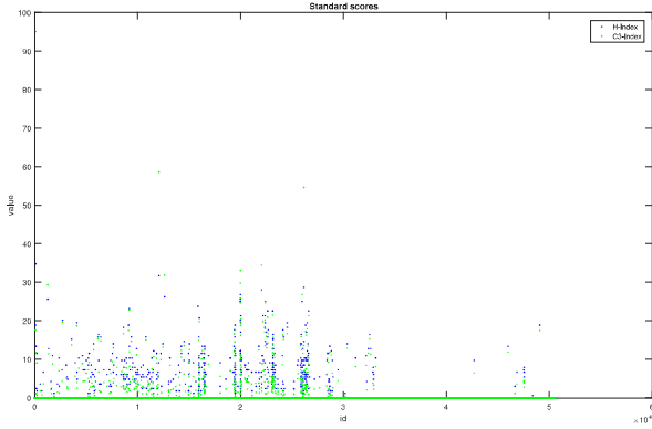
Figure 4: h -index versus C^3 -index value distribution per author ID.
