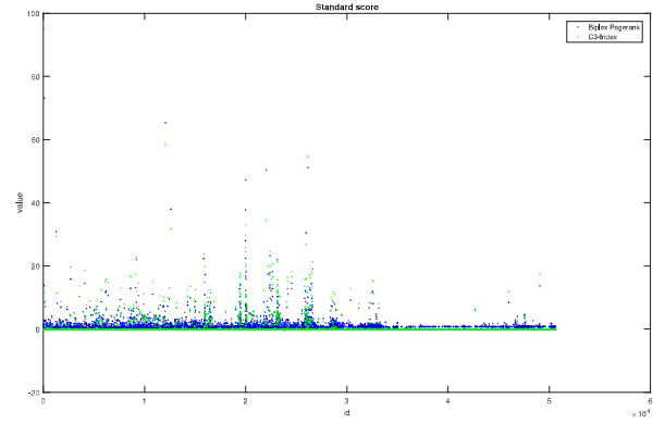
Figure 2: Biplex PageRank versus C^3 -index value distribution and correlation per author ID.
