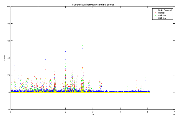
Figure 6: C^4 -index versus the other competitors' value distribution per author ID.
