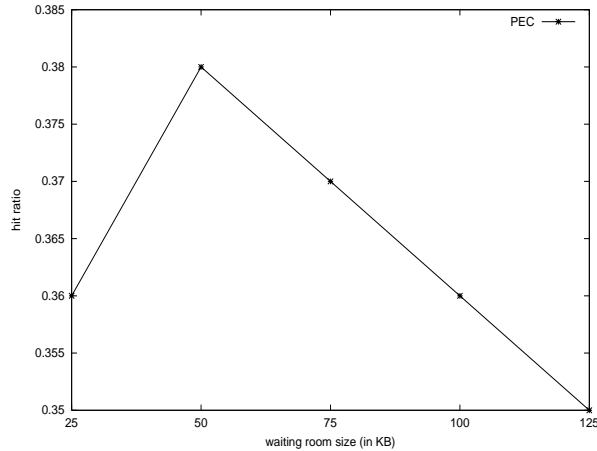
Fig. 7. Hit ratio w.r.t. Waiting Room size.
