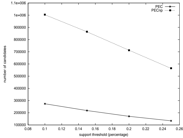
Fig. 8. Number of candidates w.r.t. support threshold
