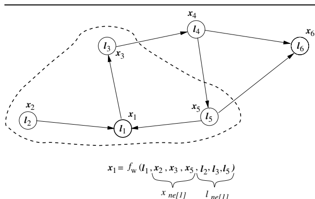
Figure 2. The dependence of state x_1 on neighborhood information.
