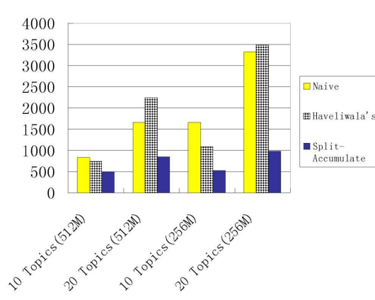
Figure 6: Running times in seconds for Topic-Sensitive Pagerank with 10 and 20 topics on 256MB and 512MB.
