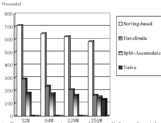
Figure 4: Running times in seconds for all four algorithms under different memory settings.
